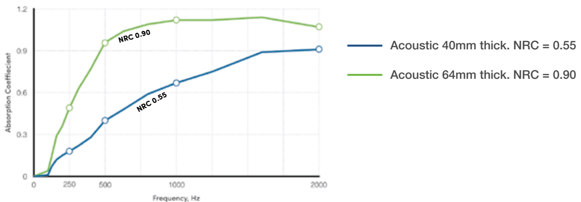
Measurement of Sound Absorption in accordance with BSEN ISO 354:2003 (Test report number C/23213/T01)
